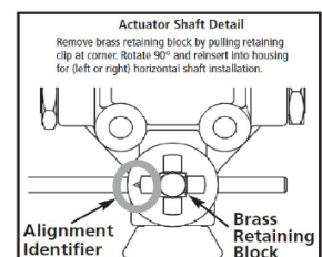
Height Control Valve Installation Instruction
